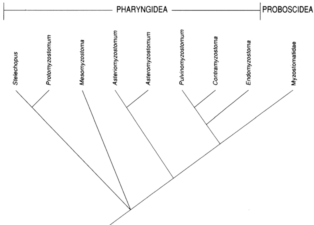
FIGURE 2. Phylogenetic relationships among the Myzostomida genera (following Grygier, 2000), based in part upon characters discussed by Jägersten (1940).
