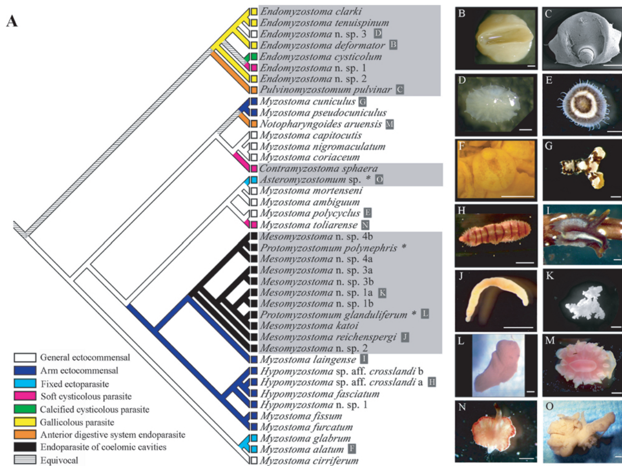
FIGURE 7. MP reconstruction of the evolution of myzostomid symbiotic lifestyles (A) and microscopic views of myzostomid species (B–O are LM views except C, which is a scanning electronic microscopy view). Grey boxes indicate members of the order Pharyngidea while all other species are members of the order Proboscidea. Asterisks indicate that the phylogenetic positions of Protomyzostomum polynephris and P. glanduliferum (parasites of ophiuroid gonads), and of Asteromyzostomum sp. (infesting the ambulacral groove of sea stars) have been estimated only from 18S rDNA data (cf. Table 4 and Fig. 6). Letters in grey frames indicate species corresponding with pictures on the right. Scale bars: 1 mm.
