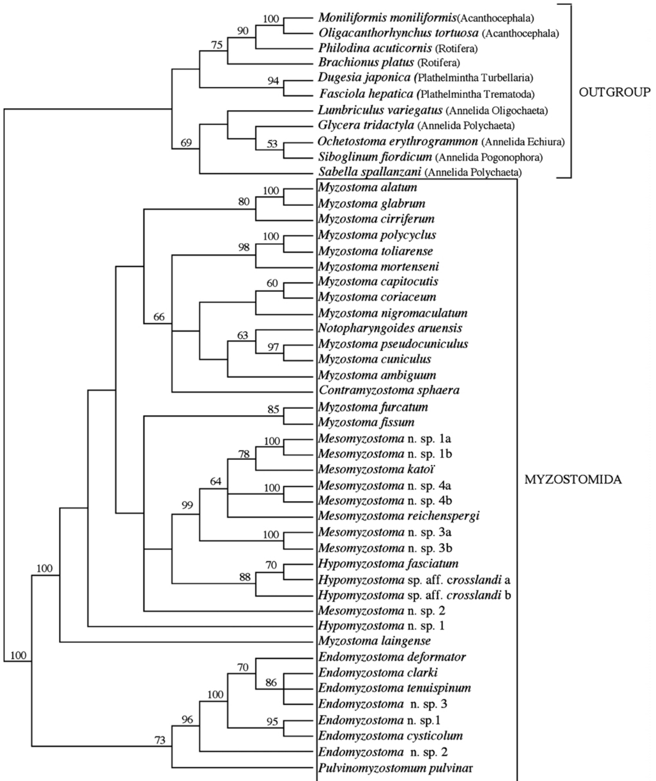
FIGURE 3. Rooting of the Myzostomida tree. Strict consensus among the six MP trees (38 ingroup taxa, 11 outgroup taxa) using the 18S rDNA alignment based on secondary structure (tree length = 2,957, CI = 0.5749, RI = 0.7602). Likelihood analyses (MetaGA and Bayesian) produced topologies similar to this one. Numbers above branches indicate bootstrap values >50% (1,000 replicates).
